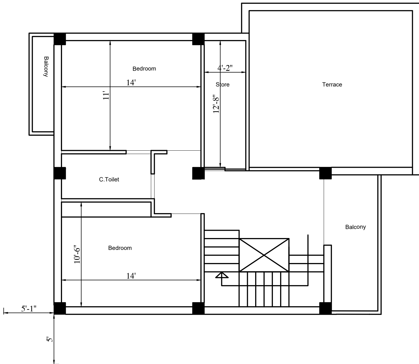
TOP FLOOR PLAN AREA: 676.83 SQ. FT
